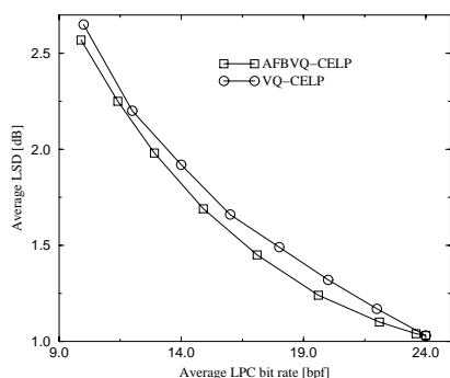
Figure 5: Comparison of AFBVQ-CELP and VQ-CELP in terms of LSD.
