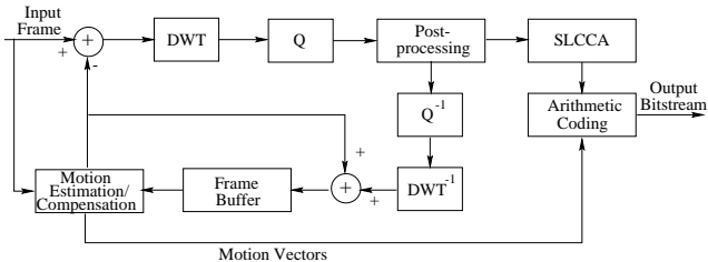
Figure 1: Block diagram of VSLCCA video coding algorithm.
