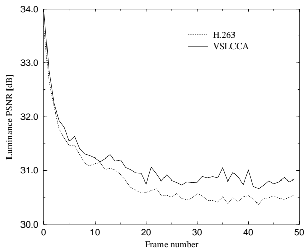
Figure 2: Performance comparison (PSNR, [dB]) between H.263 and VSLCCA for the luminance component of the “Container Ship” sequence at 5 fps, 10 kbps.
